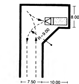
⑨ Hammerhead turn in very tight space
